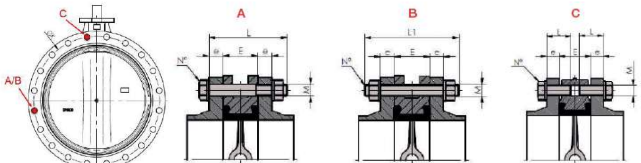
Additional 4 screws on both sides for the centring holes at DN 450 and DN 700-1600
