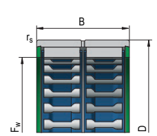
RNA69.A, F > 40 mm
